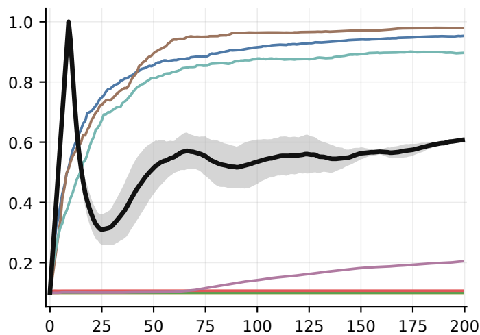
CIFAR-10
