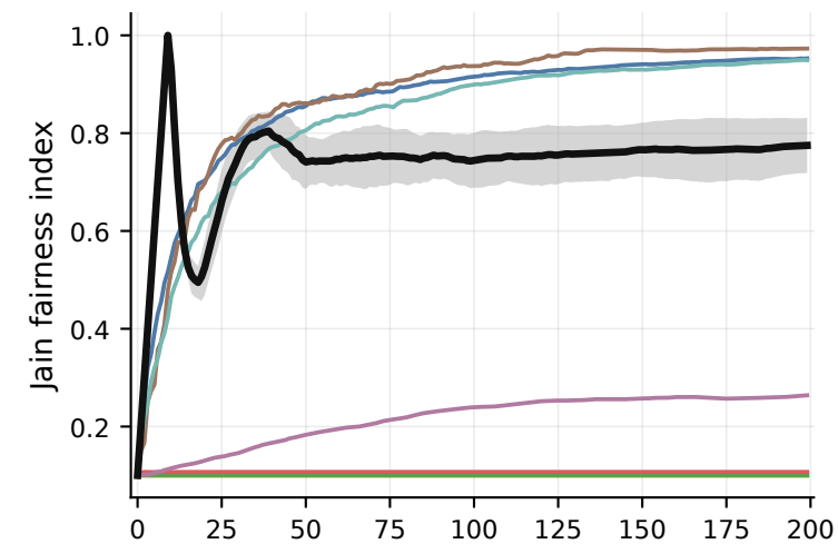
Fashion-MNIST
