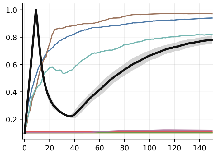
CIFAR-100
